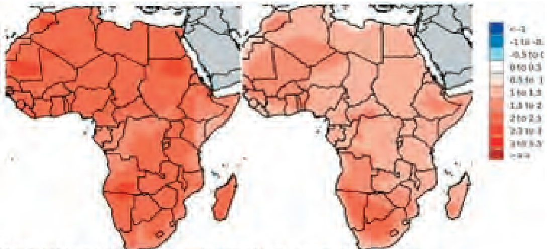
Fig. 2: Maps showing changes in normal annual maximum temperature for Sub-Saharan Africa between 2000 and 2050
